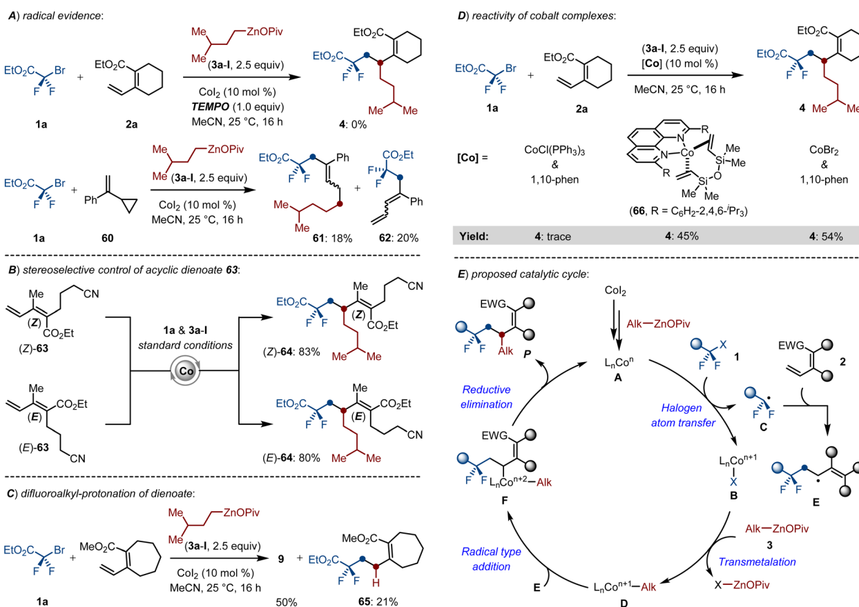
Scheme 6 Mechanistic studies.
