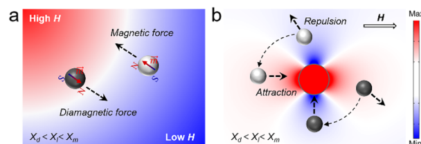
Fig. 2 (a) Schematic illustration of positive magnetophoresis and negative magnetophoresis. A magnetic object ( \chi_m > \chi_l ) experiences a magnetic force, moving towards an area of the field maximum; a diamagnetic object (black sphere, \chi_d < \chi_l ) experiences a diamagnetic force, moving towards an area of the field minimum. (b) Schematic illustration of the assembly behaviour of a magnetic object and a diamagnetic object under a gradient magnetic field.
