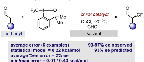
Fig. 8 Applying the secondary amine regression model to predict reaction outcomes involving copper catalyzed intermediates. (A) Assessing prediction capabilities with the arylation of aldehydes. (B) Effective prediction of trifluoromethylation reactions.
