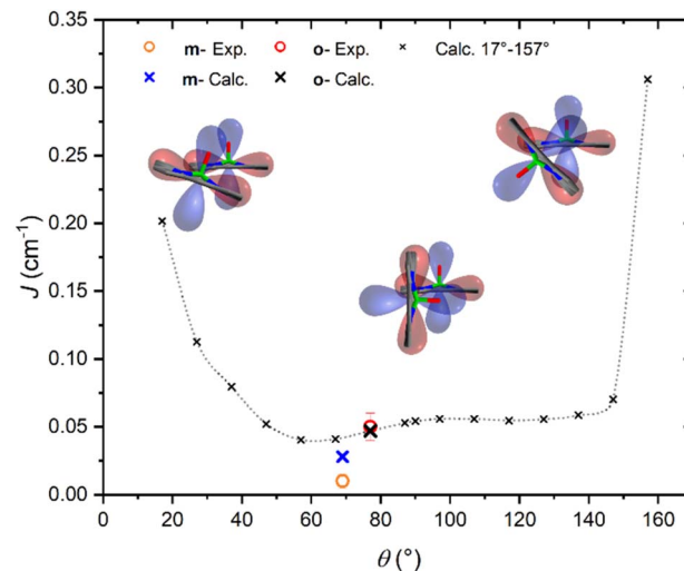
Fig. 4 Magneto-structural correlation of the exchange parameter J ( \text{cm}^{-1} ), vs. \theta ( ^\circ ). The in-plane sp and out-of-plane \pi densities of the two porphyrins are sketched by red and blue lobes, respectively. The black line across the red density indicates the porphyrin planes. Large crosses refer to values computed for the two crystallographic structures, while small crosses refer to simulated geometries obtained varying the tilting angle in o - [\text{VO}(\text{TrPP})]_2 .
