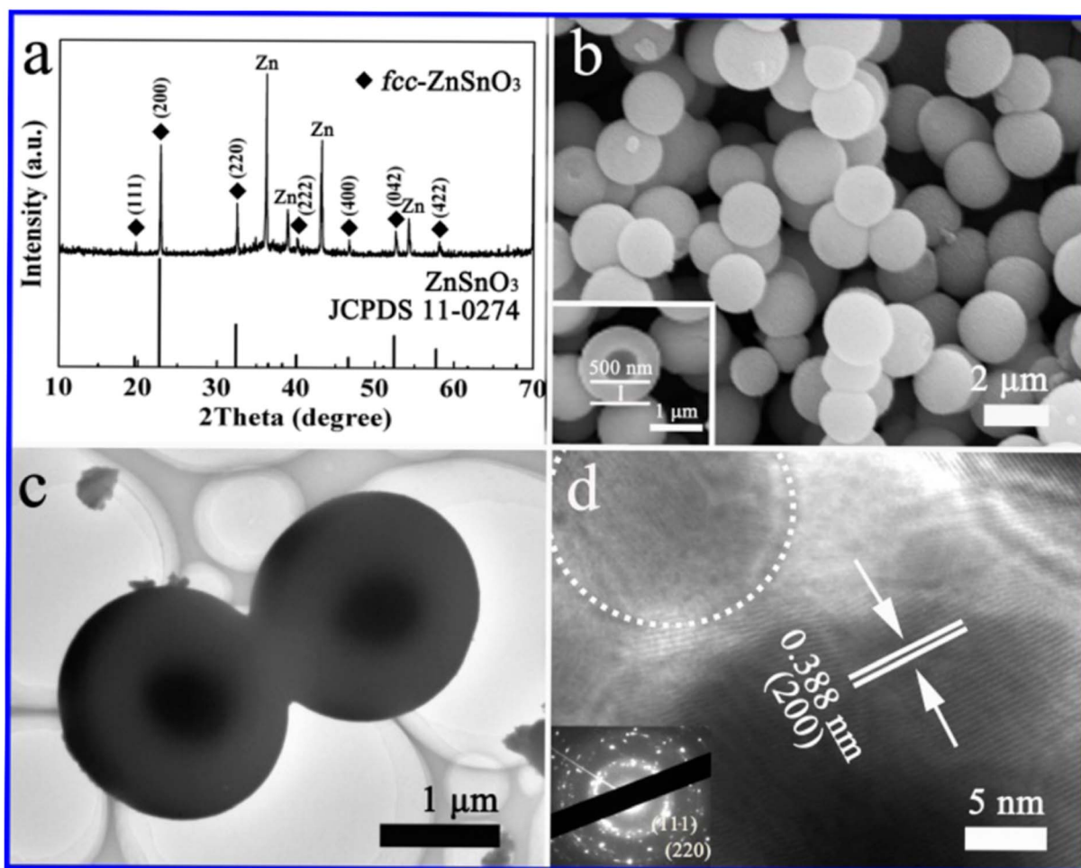
Fig. 8 (a) XRD pattern, (b) SEM image, (c) TEM image, and (d) HRTEM image of \text{ZnSnO}_3 hollow microspheres. 90
