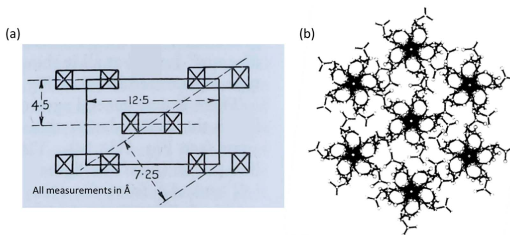
Fig. 9 Crystallographic models of NC proposed by (a) Miles in 1955 (orthorhombic) and (b) Happey et al. in 1978 (monoclinic, showing the now disputed five-fold axis). Illustrations reproduced from (a) ref. 47 , copyright Imperial Chemicals Industry 1955 and (b) ref. 70 with permission from Elsevier, copyright 1978.
