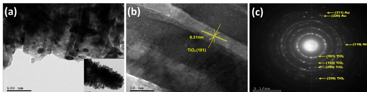
Fig. 6 (a and b) HRTEM images of Au 30 /Ni 20 /TiO 2 NTs and (c) SAED patterns of photoanode.
