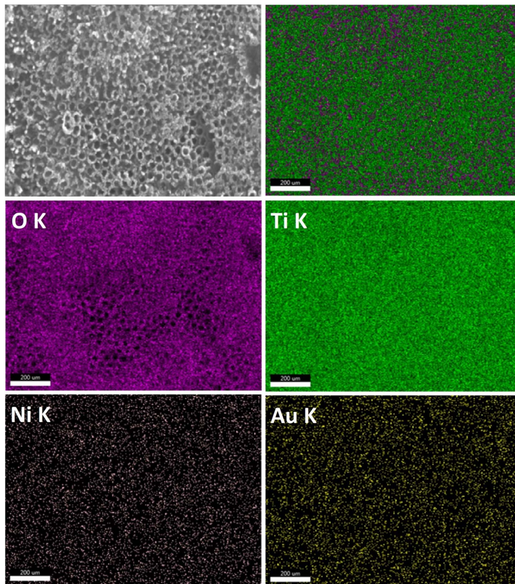
Fig. 5 The EDS elemental mapping of Au 30 /Ni 20 /TiO 2 NTs.
