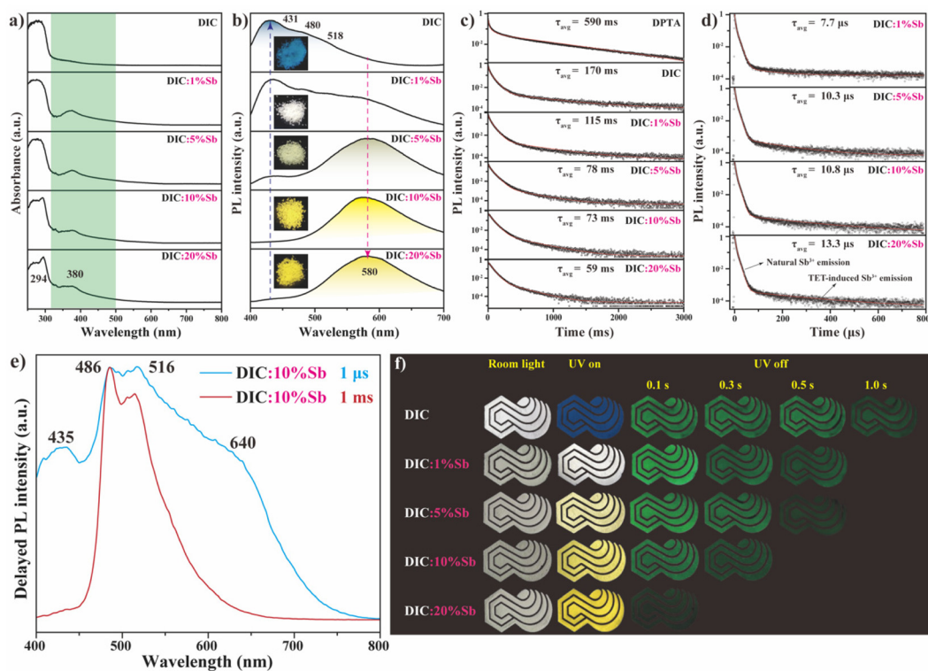
Fig. 4 (a) UV-vis diffuse reflectance spectra and (b) PL spectra of DIC: x % Sb. (c) TRPL of DIC: x % Sb at (c) 518 nm ( \lambda_{\text{exc}} = 365 nm) and (d) 580 nm ( \lambda_{\text{exc}} = 365 nm). (e) Delayed PL spectra of DIC:10% Sb at 1 \mu s and 1 ms. (f) Digital pictures of the “ \infty /CO” pattern filled with DIC: x % Sb powders under natural room light and UV irradiation and with the UV irradiation switched off.
