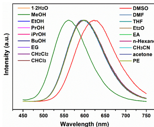
Fig. 6 Emission spectra of 1\cdot 2\text{H}_2\text{O} on exposure to MeOH, EtOH, PrOH, iPrOH, BuOH, EG, \text{CH}_2\text{Cl}_2 , \text{CHCl}_3 , DMSO, DMF, THF, \text{Et}_2\text{O} , EA, n -hexane, \text{CH}_3\text{CN} , acetone and PE under 340 nm excitation.
