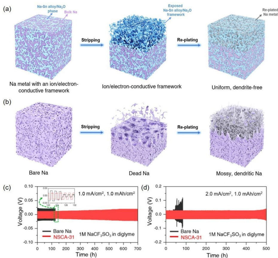
Fig. 19 Rapid and uniform Na + stripping and dendrite-free Na + plating on Na metals with ion/electron conductive frames. (b) Slow/uneven Na + stripping and dendritic Na + plating on bare Na metal. Cycling performance of symmetrical cells with bare Na and NSCA-31 electrodes with a capacity of 1.0 mA h cm -2 and the current densities of (c) 1.0 mA cm -2 and (d) 2.0 mA cm -2 . 189 (Reprinted with permission from ref. 189. Copyright 2019 Elsevier Ltd.).
