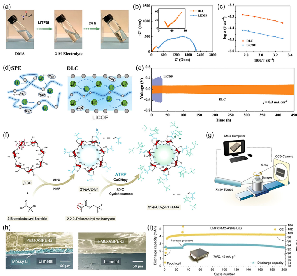
Fig. 17 (a) In situ solidification process of the DMA@LiTFSI electrolyte. (b) EIS image of SS|SSE|SS symmetric cells. (c) Ionic conductivities of pristine LiCOF and DLC SSEs. (d) Schematic illustration of the \text{Li}^+ -transport pathways in conventional SPE and DLC. (e) Comparison of cycling performance of Li|SSE|Li symmetric cell using pristine LiCOF and DLC electrolytes. Reproduced with permission. 186 Copyright 2022, Wiley-VCH GmbH. (f) Synthetic scheme of 21- \beta -CD-g-PTFEMA. (g) Schematic illustration of the working principle of X-ray tomography. (h) SEM images (side view) of the cycled Li|PEO-ASPE-Li|Li and Li|FMC-ASPE-Li|Li symmetric cells. (i) Cycling stability of LMFP|FMC-ASPE-Li|Li pouch cell. Reproduced with permission. 187 Copyright 2022, Nature Publishing Group.
