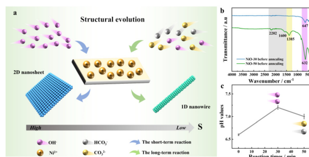
Fig. 2 (a) Schematic diagram of the evolution mechanism of the NiO homostructure with nanosheets and nanowires; (b) FTIR spectra of NiO-30 and NiO-50 films before annealing; (c) pH change curve as a function of different hydrothermal times.
