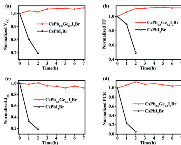
Fig. 8 Stability tests of CsPb 0.8 Ge 0.2 I 2 Br and CsPbI 2 Br PSCs upon the storage in the ambient atmosphere (50–60% RH): (a) V oc , (b) FF, (c) J sc , and (d) PCE. Reproduced from ref. 80 with permission from Wiley-VCH. Copyright 2018.
