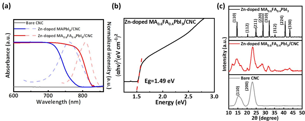
Fig. 2 (a) Absorbance spectra of bare CNC, Zn-doped \text{MA}_{0.6}\text{FA}_{0.4}\text{PbI}_3/\text{CNC} , and Zn-doped \text{MAPbI}_3/\text{CNC} papers and fluorescence spectra of Zn-doped \text{MA}_{0.6}\text{FA}_{0.4}\text{PbI}_3/\text{CNC} and Zn-doped \text{MAPbI}_3/\text{CNC} papers (dashed lines). (b) Tauc plot of the Zn-doped \text{MA}_{0.6}\text{FA}_{0.4}\text{PbI}_3/\text{CNC} paper. (c) XRD patterns of bare CNC, Zn-doped \text{MA}_{0.6}\text{FA}_{0.4}\text{PbI}_3/\text{CNC} papers, and Zn-doped \text{MA}_{0.6}\text{FA}_{0.4}\text{PbI}_3 films.
