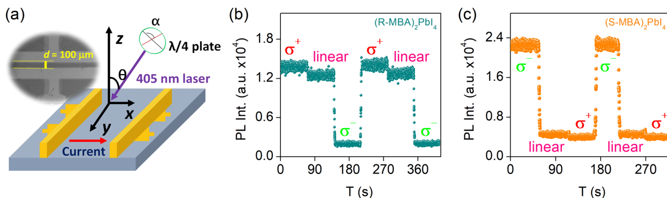
Fig. 2 (a) The schematic drawing of the lateral device configuration Au/chiral LHP/Au. The inset image shows the channel length of approximately 100\ \mu\text{m} . (b) and (c) are the variations of the PL intensities due to the photo switches among the left-, linear and right-circularly polarized photoexcitation for (R-MBA)_2PbI_4 and (S-MBA)_2PbI_4 , respectively. The photoexcitation wavelength and the laser power were 405 nm and 90 mW, respectively.
