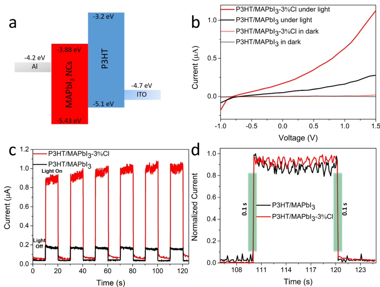
Fig. 5 Schematic diagram of the energy levels (a) or work function of Al, MAPbI 3 NCs, P3HT, and ITO in the PD devices. The current–voltage ( I–V ) curves (b) of the P3HT/MAPbI 3 and P3HT/MAPbI 3 -3%Cl based PDs (device area: 0.1 cm 2 ) in dark and under weak natural light (power density: 30 mW cm -2 ). Time-dependent photoresponse characteristics (c) of P3HT/MAPbI 3 and P3HT/MAPbI 3 -3%Cl based PDs at a bias of +1 V under weak natural light. The rise ( t_{\text{on}} ) and fall time ( t_{\text{off}} ) (d) of P3HT/MAPbI 3 and P3HT/MAPbI 3 -3%Cl based PDs.
