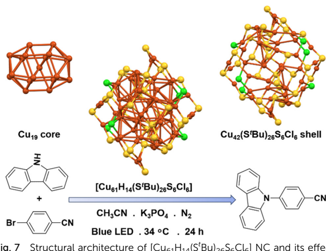
Fig. 7 Structural architecture of [Cu 61 H 14 (S i Bu) 26 S 6 Cl 6 ] NC and its effectiveness towards photocatalytic C–N coupling reaction. Cu displayed in brown color; S displayed in yellow color and Cl displayed in green color. Other ligands were removed for clarity. Hydrides were not detected by SCXRD. Figure created based on the cif file deposition of ref. 73.
