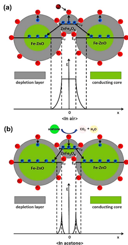
Fig. 14 Schematic diagram of the structure and band for the \text{ZnFe}_2\text{O}_4/\text{Fe-ZnO} nanocomposite-based sensor (a) in air and (b) in acetone (reproduced with permission from ref. 90. Copyright 2020 Elsevier).
