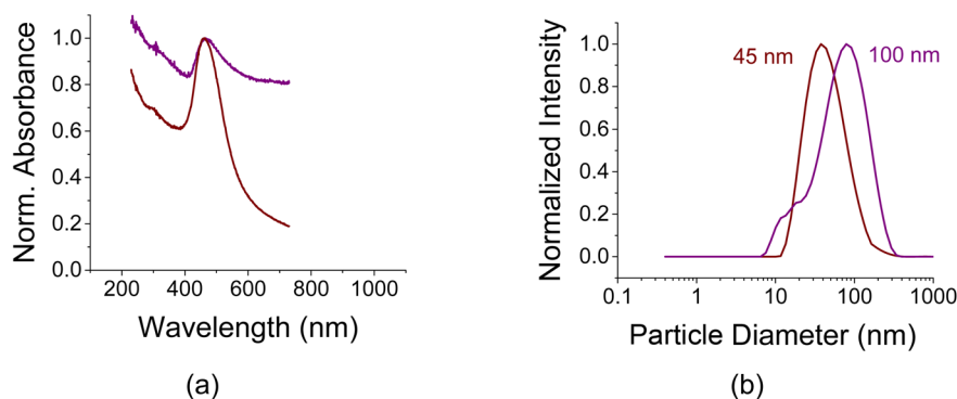
Fig. 1 (a) Absorbance (normalized such that the peak equals unity) for ligand-coated, small size (wine color) and aggregates (purple color) of AuNPs. Both were suspended in water. The plasmonic absorption is clearly seen; the aggregate peak is a bit red-shifted and broader compared to the small particles' peak. The increase in absorption towards the UV spectrum is attributed to increased scattering. (b) The corresponding DLS data show the two particle sizes used in the experiments.
