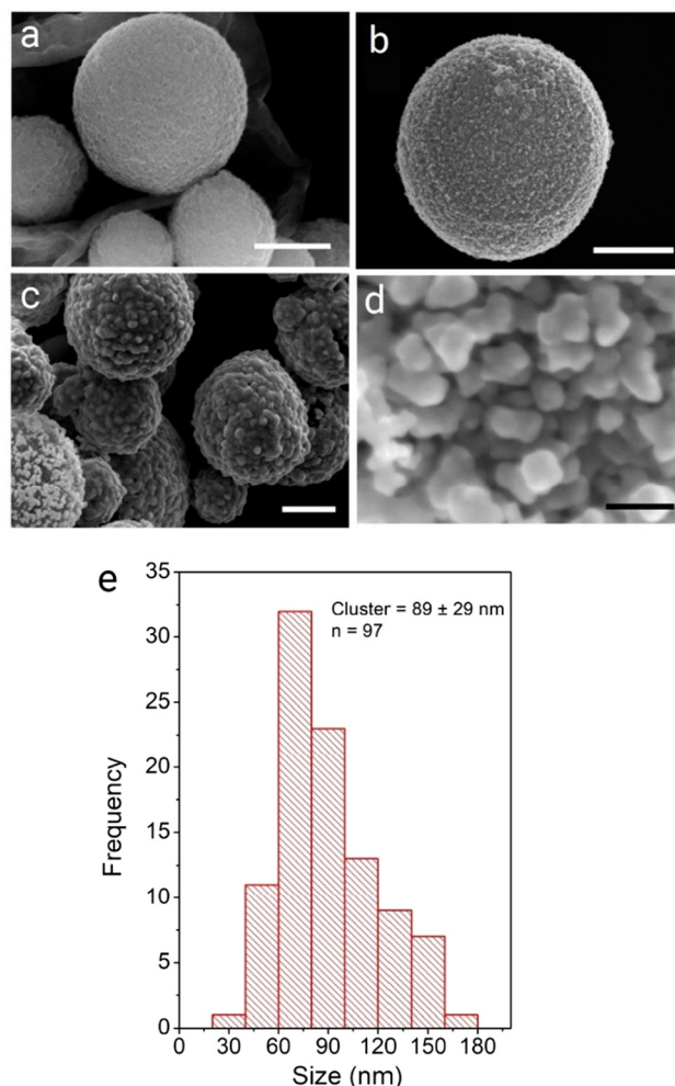
Fig. 1 SEM micrographs of precursor and composite systems prepared using approach 1: (a) o- C_{\mu}P , (b) C_{\mu}P -AuNP(DMAP) and (c and d) roughened composites C_{\mu}P -AuNP-1 . Scale bars show (a–c) 500 nm and (d) 50 nm.
