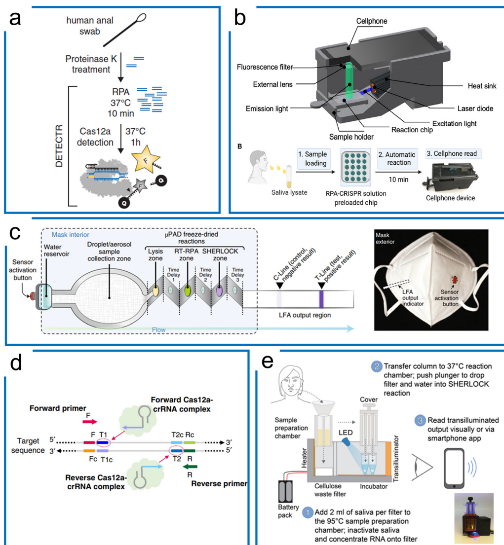
Fig. 6 The RPA-based Cas12 systems for nucleic acid detection. (a) The DETECTR system of Cas12a diagnostics for HPV viral detection, the sample was treated with proteinase K, followed by RPA, and then the targets were detected by Cas12a ribonucleoprotein for trans -cleavage of the ssDNA reporters. The figure was reproduced from ref. 44 with permission from the American Association for the Advancement of Science, copyright 2018. (b) A miniaturized system with cell phone readout using the RPA-Cas12a system that allows sensitive and quantitative readout of saliva CRISPR-FDS assays at sites. Sample preparation, amplification, and detection are all combined in one device. The figure was reproduced from ref. 113 under Creative Commons Attribution License from the American Association for the Advancement of Science, copyright 2021. (c) The RPA-Cas12a diagnostics with paper microfluidics in a mask. Once the water reservoir was opened, the target was driven by the capillary force of paper microfluidics through different folded layers for three purposes including sample lysis, RT-RPA amplification, and Cas12a-based detection. All these chemicals associated with these purposes were lyophilized reagents in the mask. The figure was reproduced from ref. 114 with permission from Springer Nature, copyright 2021. (d) A one-pot RPA-Cas12a assay with two targeting sites of crRNAs for enhanced sensitivity of Cas12a diagnosis of COVID-19. After RPA amplification, the amplicons can be targeted using two crRNAs to boost the sensitivity higher compared to the conventional one-crRNA method. The figure was reproduced from ref. 122 under Creative Commons Attribution License from Springer Nature, copyright 2020. (e) A portable device with enhanced one-pot Cas12a and RPA reaction for SARS-CoV-2 and related variants' detection. The target sample was firstly treated with a high temperature for sample preparation, following liquid transfer to another lyophilized power tube to perform the one-pot RPA-Cas12a reaction. Sample preparation, RPA amplification, and Cas12a detection steps were integrated into a small device with a mobile phone readout. The figure was reproduced from ref. 125 under Creative Commons Attribution License from the American Association for the Advancement of Science, copyright 2021.
