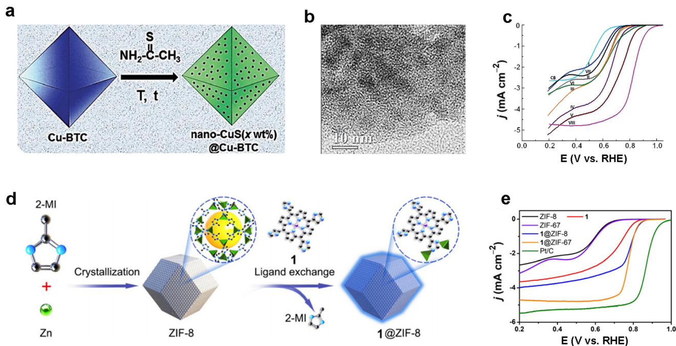
Fig. 11 MOF-based ORR electrocatalysts. (a) Schematic diagram of the synthesis of \text{CuS}(x \text{ wt}\%)@Cu\text{-BTC} nanoparticles; (b) TEM images of \text{nano-CuS}(28 \text{ wt}\%)@Cu\text{-BTC} ; (c) LSV curves of \text{nano-CuS}(28 \text{ wt}\%)@Cu\text{-BTC} and other samples for ORR tests in \text{O}_2 -saturated 0.1 M KOH, rotation rate: 1600 rpm. Reproduced with permission. 97 Copyright 2016, Wiley-VCH; (d) schematic diagram of the preparation of 1@ZIF\text{-8} ; (e) LSV curves of 1@ZIF\text{-8} and other samples for ORR tests in \text{O}_2 -saturated 0.1 M KOH, rotation rate: 1600 rpm. Reproduced with permission. 98 Copyright 2021, Wiley-VCH.
