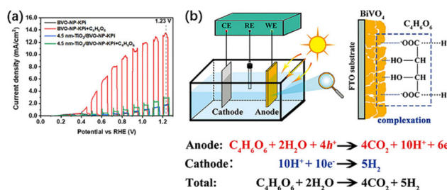
Fig. 7 (a) Current density versus potential curves of BVO-NP and 4.5 nm \text{TiO}_2 /BVO-NP photoanodes in potassium phosphate (KPI) and KPi + 0.5 M \text{C}_4\text{H}_6\text{O}_6 solutions under AM 1.5G illumination or in the dark. (b) Schematic illustration of the detailed reaction process in the \text{BiVO}_4 PEC fuel cell system. Adapted from ref. 58 with permission from John Wiley and Sons, copyright 2022.
