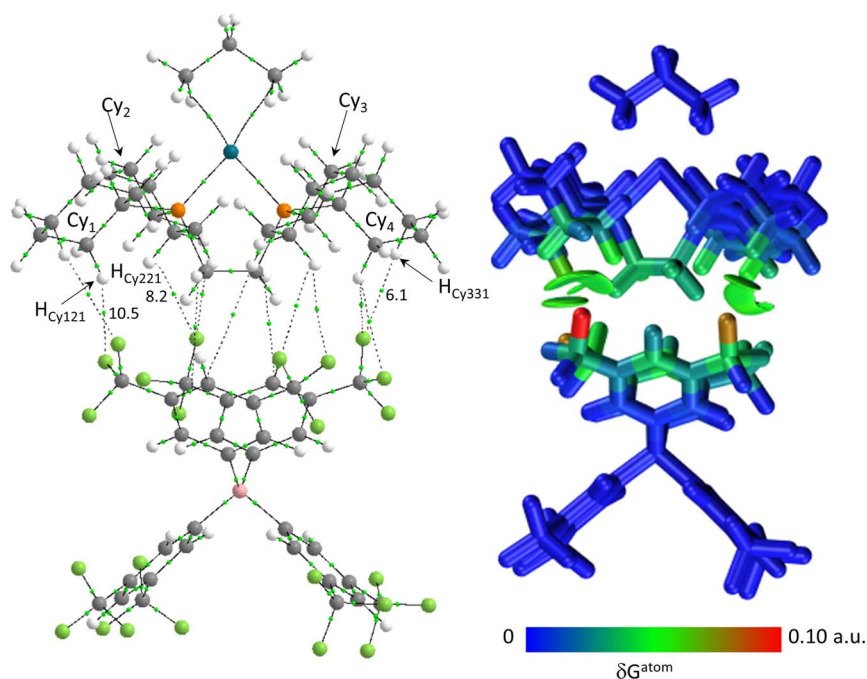
Fig. 9 (a) QTAIM molecular graph with the bottom anion in [1-propane][BAR F 4 ] with BCPs in green and showing selected atoms and BCP electron densities (a.u. × 10 −3 ). Bond paths with \rho(r) < 0.001 a.u., intramolecular bond paths and ring critical points (RCP) are omitted for clarity. (b) IGMH plot where the cation and anion are defined as separate fragments. Sign( \lambda_2 ) \rho -coloured isosurfaces are plotted with \delta G^{\text{inter}} = 0.003 a.u. and atoms are coloured by \delta G^{\text{atom}} .
