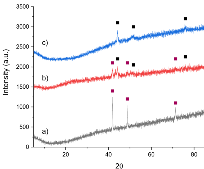
Fig. 1 XRD patterns of \text{Co}_3\text{CuN} : (a) pre-reaction, (b) post-reaction with 3 : 1 \text{ H}_2/\text{N}_2 at 200^\circ \text{C} and 250^\circ \text{C} and (c) post-reaction with 3 : 1 \text{ H}_2/\text{N}_2 at 300^\circ \text{C} and 400^\circ \text{C} . (■) \text{Co}_3\text{CuN} and (■) \text{Co}_3\text{Cu} .
