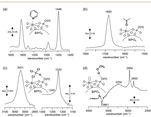
Fig. 8 Difference IR spectra for (a) pyridine-, (b) acetone-, (c) chloroform-, and (d) CH 3 OH-adsorbed BiPO 4 -DEG at 25 °C.
