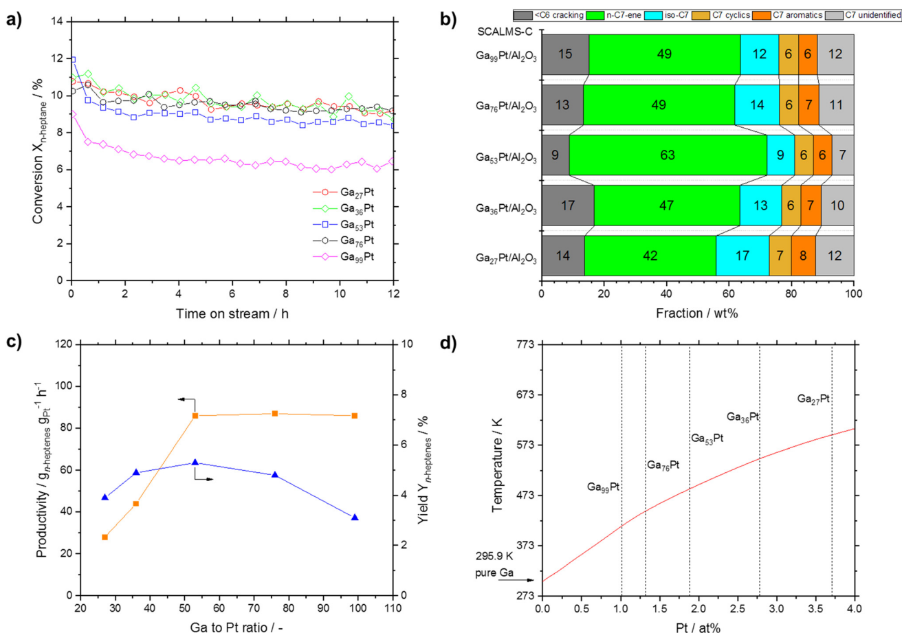
Fig. 12 a) Conversion over time in n\text{-heptane} dehydrogenation as function of the Ga-Pt ratio (all samples prepared according to the SCALMS-C protocol). b) Respective selectivity (at TOS = 12 h) in n\text{-heptane} dehydrogenation. c) Productivity and yield of heptenes obtained. d) Section of the Ga-Pt phase diagram according to Okamoto with liquidus line shown in red. 51 Reaction conditions: 703 K, atmospheric pressure, 2.5 mL catalyst, H_2/n\text{-heptane} = 8/1 , 0.062 \text{ g min}^{-1} n\text{-heptane} , 118.87 \text{ mL}_N \text{ min}^{-1} H_2 , 14.86 \text{ mL}_N \text{ min}^{-1} He , 3320 \text{ mL}_{\text{gas}} \text{ g}_{\text{cat-bed}}^{-1} \text{ h}^{-1} GHSV, \sim 1.1 s residence time ( \tau ).
