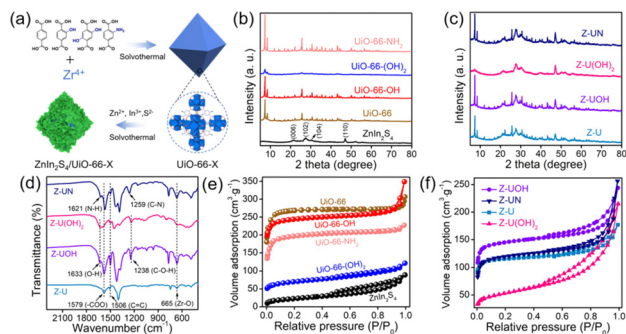
Fig. 2 Preparation diagram of \text{ZnIn}_2\text{S}_4/\text{UiO}-66\text{-X} hybrids (a), XRD patterns (b and c) and \text{N}_2 adsorption–desorption isotherms (e and f) of UiO-66- \text{NH}_2 , UiO-66-(OH) _2 , UiO-66-OH, UiO-66, \text{ZnIn}_2\text{S}_4 , Z-UN, Z-U(OH) _2 , Z-UOH and Z-U, FTIR spectra of Z-UN, Z-U(OH) _2 , Z-UOH and Z-U (d).
