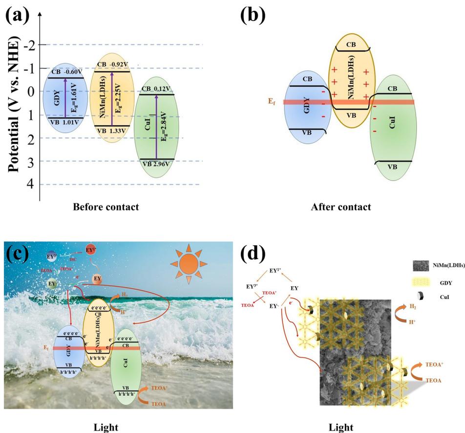
Fig. 11 (a and b) Double S-scheme heterojunction mechanism towards the charge transfer between CuI, GDY and NiMn(LDHs) before and after contact in darkness and under illumination. (c and d) Possible hydrogen evolution mechanism diagram for the GDY/CuI/NiMn(LDHs) photocatalyst.
