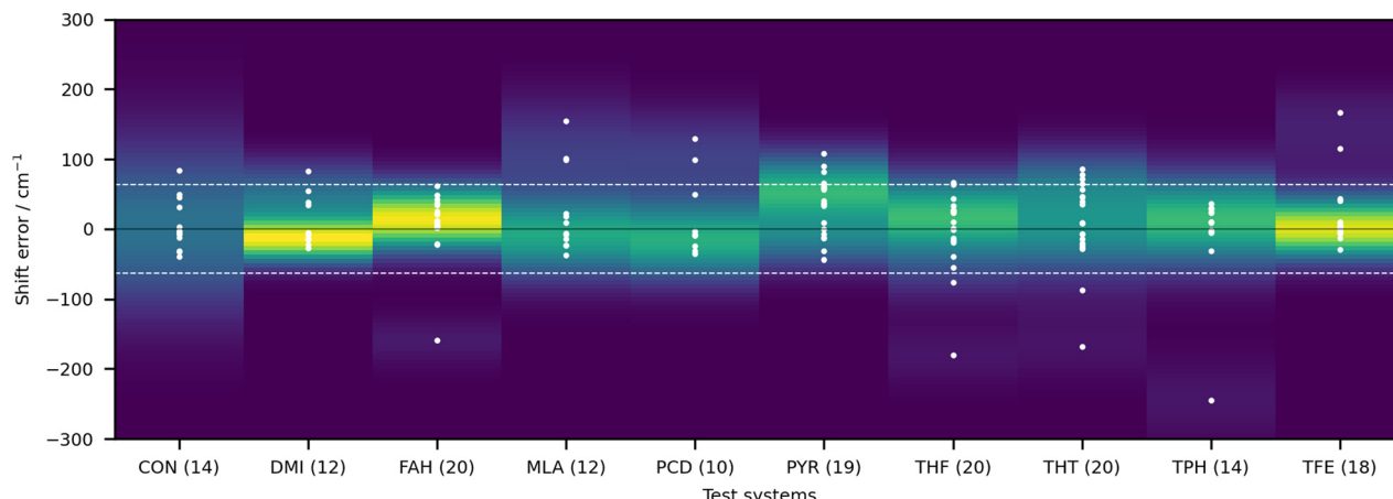
Fig. 3 Deviations of the submitted OH stretch shifts relative to the measured experimental values (raw values) in \text{cm}^{-1} for the 10 test systems. A positive error means that the predicted wavenumber downshift from the monomer is too large. Each value is represented as a white dot (only one value is outside of the visualisation window, AC1 submission for CON, with an error of 460.5 \text{ cm}^{-1} ). The color coding of the graph is provided by the probability density function of the error for each system. Yellow indicates larger density values, dark blue low density. The bandwidth selection has been made with Scott's rule. 33 The dotted line delimits the RMSD range of the null hypothesis ( 62.3 \text{ cm}^{-1} ), obtained as described in the text.
