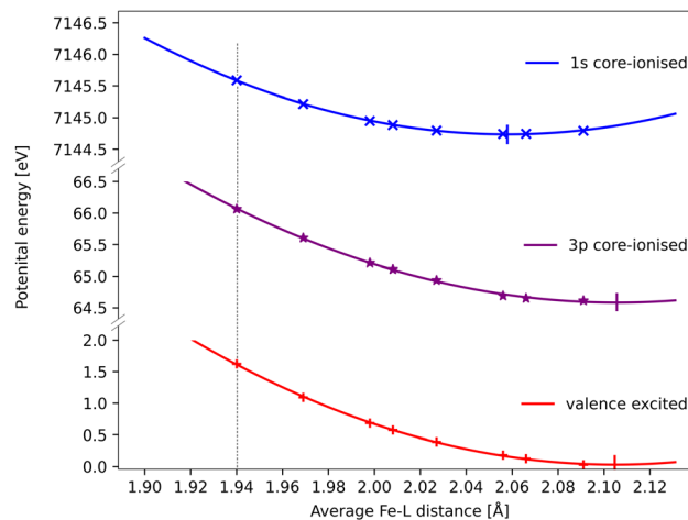
Fig. 9 RAS energies as a function of the Fe–ligand distance for the {}^3\text{MC} valence state, the lowest {}^3\text{MC} 1s-hole state, and the {}^3\text{MC} 3p-hole state with the highest transition probability from that 1s-hole state. The grey dotted vertical line at 1.940 \text{ \AA} represent the average Fe–L bond length for the GS geometry. Quadratic PES fits give minima at 2.06 \text{ \AA} , 2.11 \text{ \AA} and 2.11 \text{ \AA} for the 1s, 3p core–hole and {}^3\text{MC} valence states and corresponding force constants of 122 \text{ eV } \text{\AA}^{-2} , 108 \text{ eV } \text{\AA}^{-2} and 117 \text{ eV } \text{\AA}^{-2} . The fit values must be considered uncertain considering deviations from quadratic behaviour, lack of data points close to the minima, and the presence of multiple local SCF minima. The force constant for the 1s hole is smaller than reported in ref. 33, likely due to a stabilization of longer Fe–ligand distances by the additional 3s orbital.
