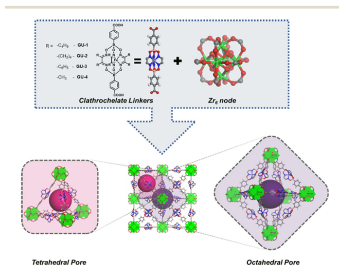
Scheme 1 Synthetic scheme of Zr-clathrochelate MOFs Zr-GU-1 to -4 and formation of octahedral and tetrahedral cavities within the framework.
