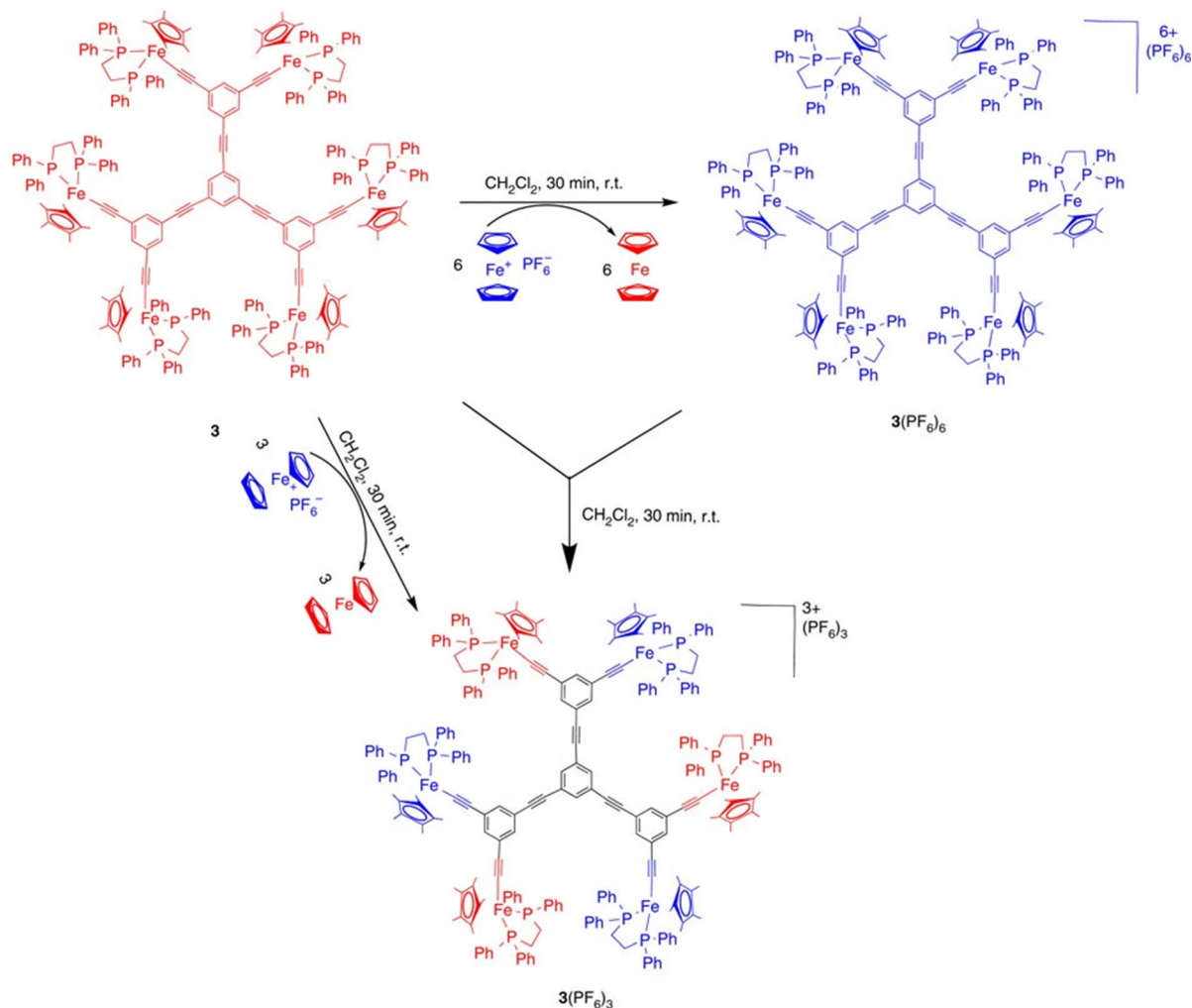
Scheme 9 Syntheses using the 17-electron ferricenium complex of both the \text{Fe}(\text{III}) and class-II mixed-valent \text{Fe}(\text{II}) – \text{Fe}(\text{III}) hexanuclear complexes. The latter can also be obtained by quantitative comproportionation between the \text{Fe}(\text{II}) and \text{Fe}(\text{III}) hexanuclear complexes. Various dendrimers containing the same mixed-valent \text{Fe}(\text{II}) – \text{Fe}(\text{III}) periphery were obtained in the same way (see Fig. 6). Blue represents \text{Fe}(\text{II}) , and red, \text{Fe}(\text{III}) . Reproduced with permission from ref.76 Copyright 2014 Springer Nature.
