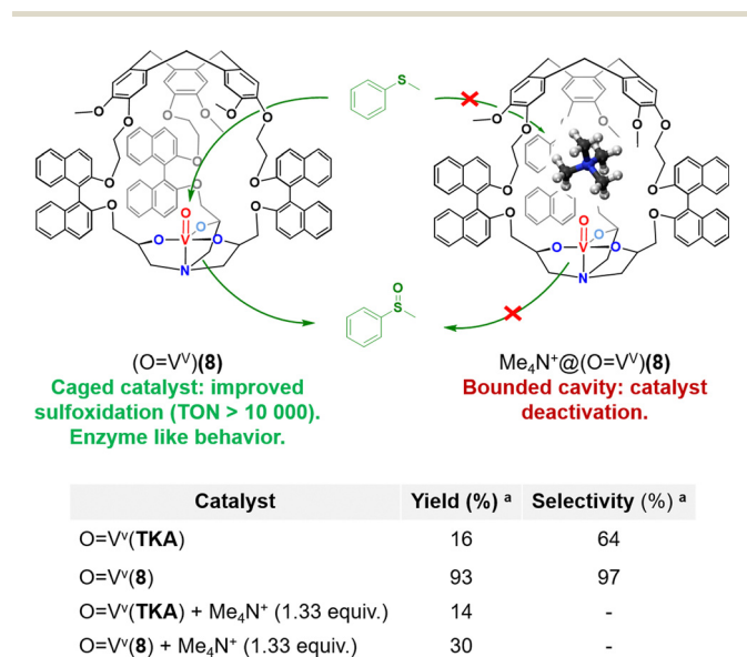
Fig. 8 (Top) Representation of the efficient sulfoxidation observed in caged oxido-vanadium catalyst ( O=V^V )( 8 ) (left), and catalyst inhibition observed upon tetramethylammonium binding in the catalyst cavity (right). (Bottom) Comparison with its open analogue devoid of the CTV cap ( O=V^V )(TKA). a Oxidation of thioanisol in the presence of the catalyst (1.5 mol%) and CHP (1.0 equiv.) for 180 min in CH_2Cl_2 at 0 °C.
