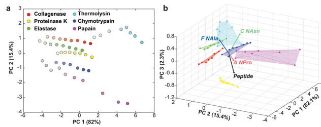
Fig. 3 (a) Two-dimensional PCA plot depicting concentration variance captured in PC1 (represented by opacity of the data points) and protease identity mapped along PC2. (b) Three-dimensional biplot showing contribution of each probe to separation.
