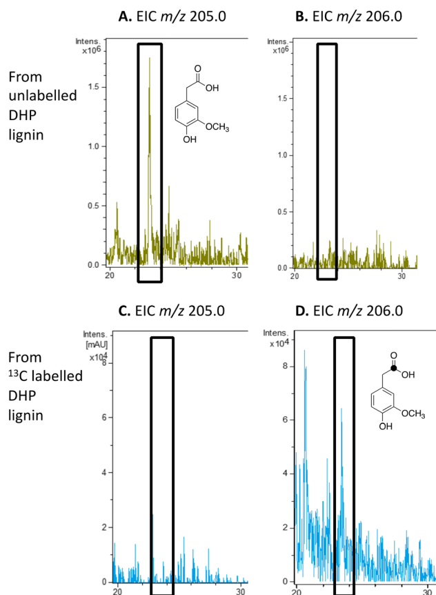
Fig. 6 Extracted ion LC-MS chromatograms for the analysis of unlabelled 4-hydroxy-3-methoxyphenylacetic acid (calculated m/z 205.0 for MNa^+ ) and ^{13}C -labelled 4-hydroxy-3-methoxyphenylacetic acid (calculated m/z 206.0 for MNa^+ ) at retention time 23.0 min, formed by treatment of unlabelled DHP lignin (panels A and B) or [ \beta - ^{13}C ]-DHP lignin (panels C and D) by Rhodococcus jostii RHA1. 4-Hydroxy-3-methoxyphenylacetic acid standard and control incubations lacking bacteria are shown in ESI ^{\dagger} Fig. S8 and S9.
