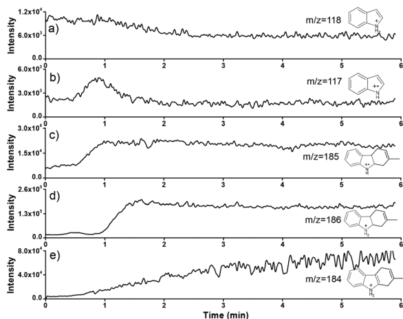
Fig. 4 Dynamic studies of different ions in confined spaces. EICs of [1 + \text{H}]^+ at m/z 118 (a), 1^{+\bullet} at m/z 117 (b), 3^{+\bullet} at m/z 185 (c), [3 + \text{H}]^+ at m/z 186 (d), and [4 + \text{H}]^+ at m/z 184 (e).
