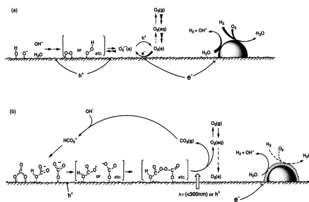
Fig. 11 Speculated reaction mechanism over Pt/TiO 2 ; (a) in water and (b) in carbonate salt aqueous solution. Reprinted with permission from Royal Society of Chemistry. 143
