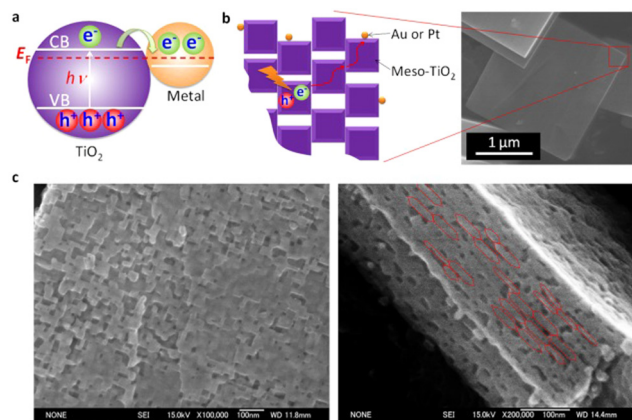
Fig. 26 Diagrammatic representation of (a) electron transfer from noble metal (Au, Pt) nanoparticles to \text{TiO}_2 upon UV light exposure. (b) The transfer of electrons on Au or Pt/ meso-TiO 2 . Meso-TiO 2 is constituted of an orderly alignment of anatase \text{TiO}_2 nanocrystals, as shown in the SEM picture in panel b. Meso-TiO 2 typically has dimensions of 2–5 \mu\text{m} and a thickness of 50–300 nm. (c) SEM pictures of the Meso-TiO 2 basal (left) and lateral (right) surfaces. Reprinted with permission from American Chemical Society. 311
