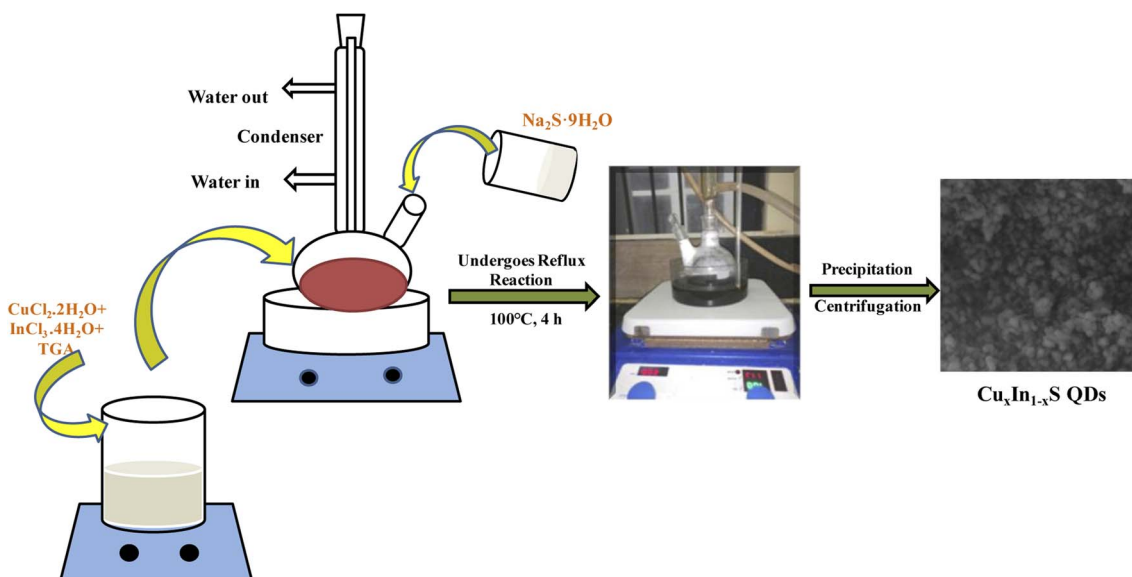
Scheme 1 Scheme for the synthesis of \text{Cu}_x\text{In}_{1-x}\text{S} QDs by varying Cu : In molar ratios via the reflux strategy.
