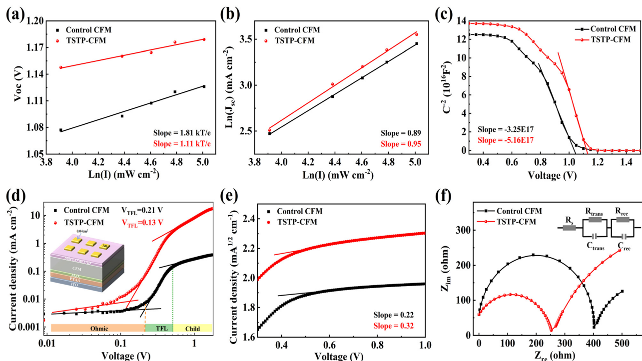
Fig. 6 (a) V_{oc} and (b) J_{sc} versus light intensity and (c) M–S plots of the control CFM and TSTP-CFM devices. (d) J – V and (e) J^{1/2} – V characteristics of SCLC measurements for hole-only devices with the architecture of ITO/PTAA/CFM (with and without TSTP treatment)/spiro-OMeTAD/Au; the inset is the device structure diagram. (f) EIS of the control CFM and TSTP-CFM devices under the illumination of 100\text{ mW cm}^{-2} ; the inset shows the equivalent electrical circuit of PSCs.
