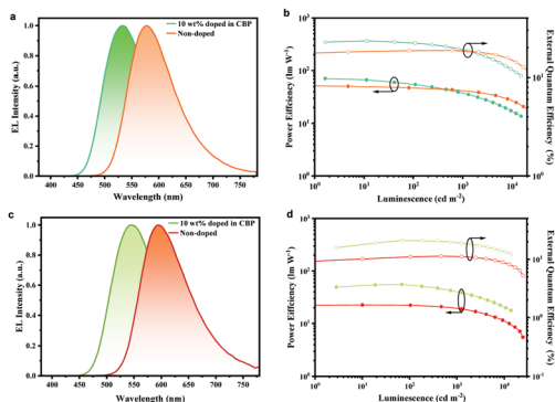
Fig. 4 EL spectra and the PE–luminance–EQE characteristics of the doped and non-doped devices based on PyPmP (a and b) and PmPmP (c and d).
