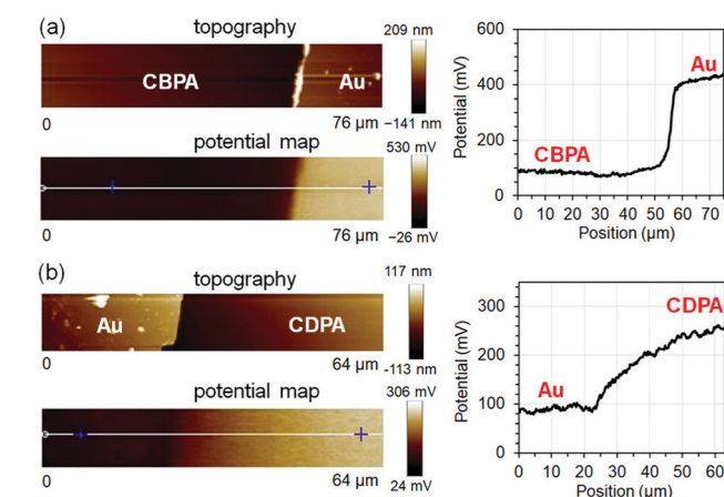
Fig. 2 Representative AFM topography image, KPFM electrostatic potential map and line scan (along the white line in the potential map) for the SAMs of CBPA (a) and CDPA (b).
