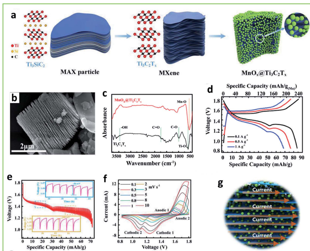
Fig. 25 (a) Schematic illustration of the synthesis of \text{MnO}_x @ \text{Ti}_3\text{C}_2\text{T}_x ; (b) SEM images of multilayered \text{Ti}_3\text{C}_2\text{T}_x ; (c) Fourier-transform infrared spectroscopy of \text{Ti}_3\text{C}_2\text{T}_x and \text{MnO}_x @ \text{Ti}_3\text{C}_2\text{T}_x ; (d) GCD profiles of \text{MnO}_x @ \text{Ti}_3\text{C}_2\text{T}_x at different current densities; (e) discharge profiles based on galvanostatic intermittent titration technique of \text{MnO}_x @ \text{Ti}_3\text{C}_2\text{T}_x -based Zn-ion battery; (f) CV curves of \text{MnO}_x @ \text{Ti}_3\text{C}_2\text{T}_x based Zn-ion battery at different scan rates; (g) schematic illustration of the nanoscale-level parallel circuitry-based on \text{MnO}_x @ \text{Ti}_3\text{C}_2\text{T}_x . (a–g) Are adapted with permission. 370 Copyright 2019, WILEY-VCH.
