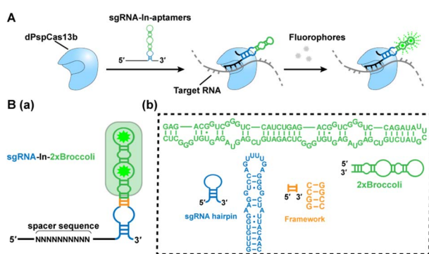
Scheme 1 Development of the CRISPR-dPspCas13b system with fluorescent RNA aptamers in sgRNA (CasFAS). (A) Schematic drawing of the CasFAS: CRISPR-dCas13 system binds with sgRNA containing fluorescent RNA aptamers and target RNA. (B) (a) Overview of sgRNA-In-2 × Broccoli designs. The structure of dCas13b sgRNA's DR loop (blue), framework (F, orange) and 2 × Broccoli (green) with DFHBI-1T (green star). (b) Modules and their sequence illustrations of sgRNA-In-2 × Broccoli.
