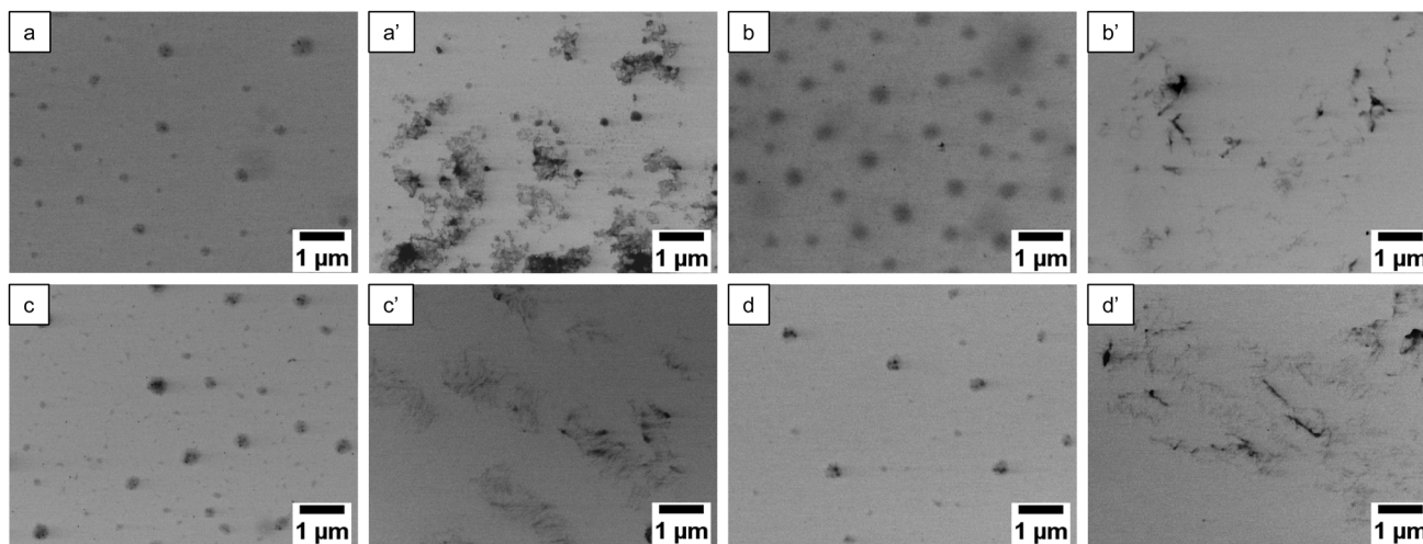
Fig. 4 STEM images of Se 1 μG before sonication of (a) 0.5, (b) 1.5, (c) 3.0, and (d) 5.0 mol% diselenide content. The images after 10 min sonication (a'), (b'), (c'), and (d') correspond to (a), (b), (c), and (d), respectively. Sonication was carried out in an ice bath at 30% amplitude for 10 min.
