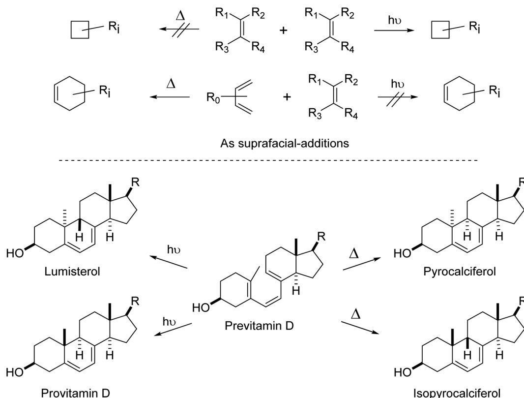
Fig. 7 (top) Examples of thermal and photochemical cycloadditions that were or were not reported in the early 1960s and earlier. These reactions depend on geometry, strain, electrostatics and polarization, Pauli repulsion and dispersion effects as well as orbital symmetry factors. 121 [2 + 2] cycloadditions are fine thermally – if the appropriate orbital symmetry-required geometries can be achieved and a high energy barrier can be overcome, or if the substituents cause significant asymmetry and the reaction proceeds by a non-Woodward–Hoffmann pathway. 122–124 (bottom) Examples of valence isomerizations in vitamin D chemistry. 125–127 Importantly, these are examples of alternating stereospecific reactions, alternation in the number of electrons involved and whether the reactions are thermal or photochemical. For more details and leading references, see Woodward and Hoffmann's major treatise of 1969 122 or a more recent historical survey. 128
