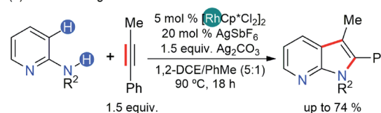
Scheme 1 Alkenylation strategies for the synthesis of 7-azaindoles.
