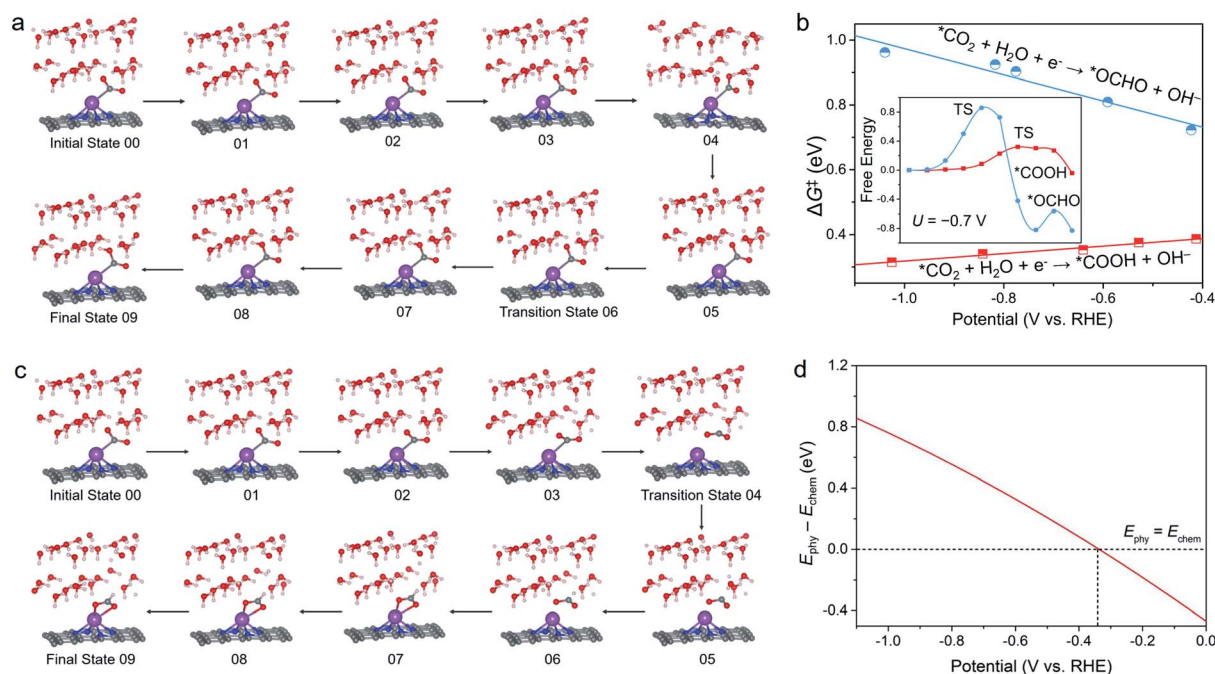
Fig. 3 Snapshots of the paths for the protonation of chemisorbed \text{CO}_2 ( ^*\text{CO}_2 ) to (a) ^*\text{COOH} and (c) ^*\text{OHCO} on the Bi-N-C SAC. (b) Kinetic barriers \Delta G^\ddagger for protonation of ^*\text{CO}_2 to form ^*\text{COOH} and ^*\text{OCHO} on the Bi-N-C SAC as a function of potential. The inset is the reaction path at U = -0.7 V. (d) Energy difference between the physisorbed \text{CO}_2 configuration and chemisorbed \text{CO}_2 configuration ( E_{\text{phy}} - E_{\text{chem}} ) of the Bi-N-C SAC as a function of potential. A more positive value of E_{\text{phy}} - E_{\text{chem}} indicates that the chemisorbed \text{CO}_2 configuration is more stable.
