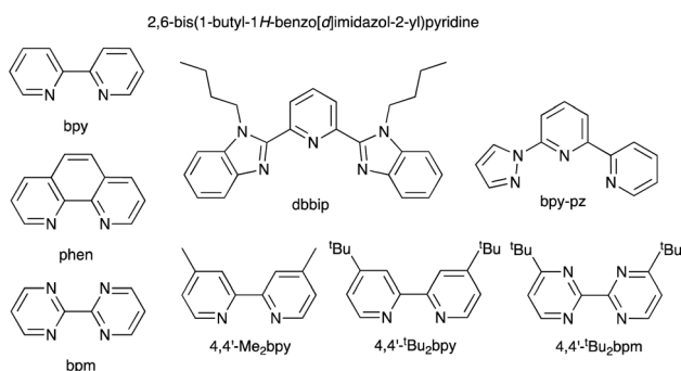
Scheme 3 Structures of bpy, phen, bpm, dbpip, bpy-pz, 4,4'-Me 2 bpy, 4,4'-tBu 2 bpy and 4,4'-di- tert -butyl-2,2'-bipyrimidine (4,4'-tBu 2 bpm).
