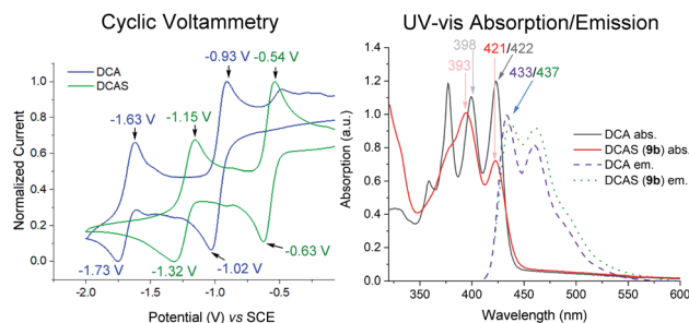
Fig. 4 Left: cyclic voltammetry of catalysts. Conditions: 0.01 M \text{DCA}/\text{DCAS} in 0.1 M n\text{Bu}_4\text{NPF}_6/\text{MeCN} , scan rate 50 \text{mV s}^{-1} . Right: UV-vis and emission spectra.
